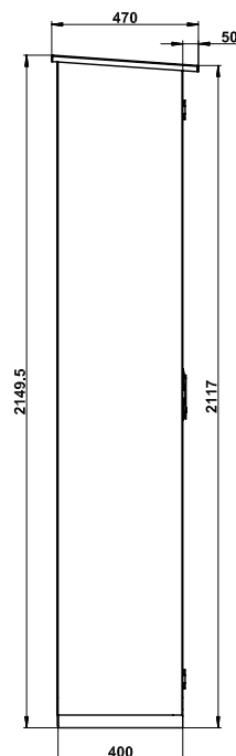
Model GOD.215.100 - widok z boku
