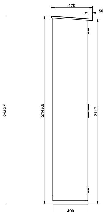
Model GOD.215.070.R - widok z boku
